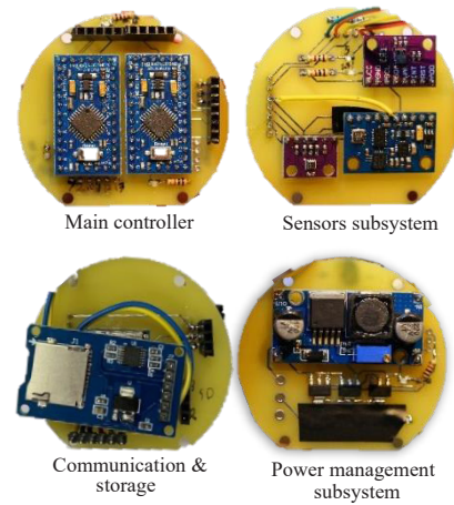
Fig. 4. AEASat floor designs.
