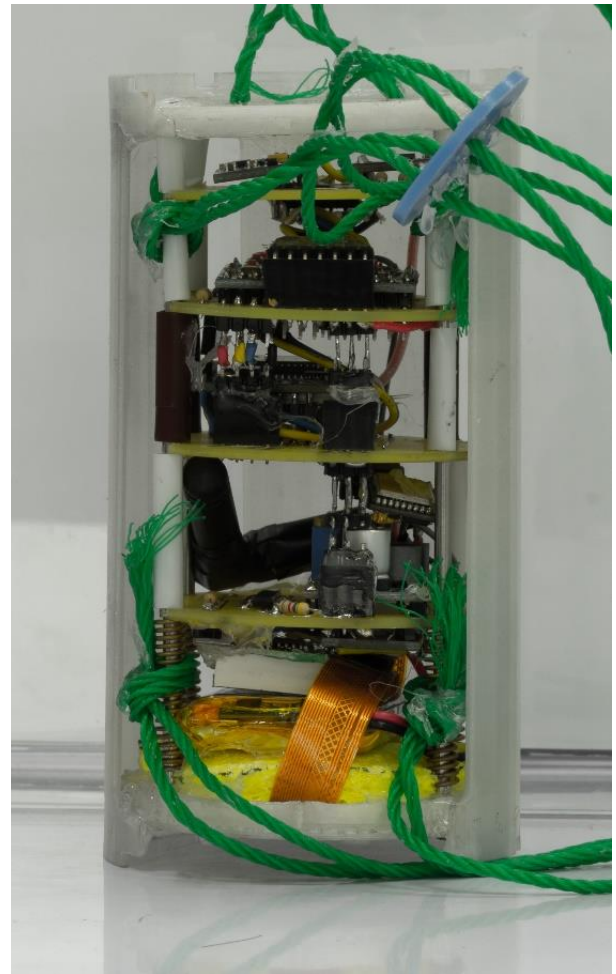
Fig. 11. The final model of AEASat.
